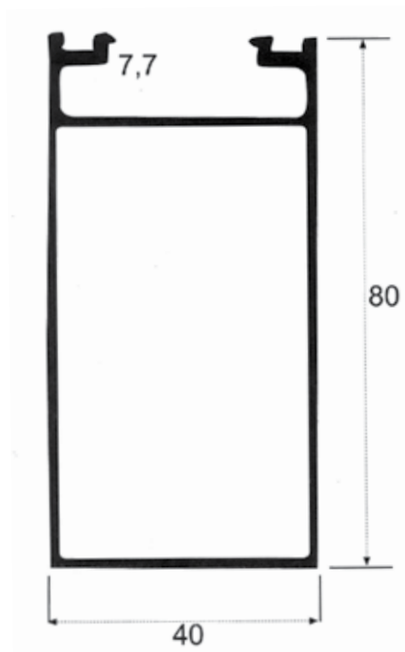
M - 30 1,210 kg/m
