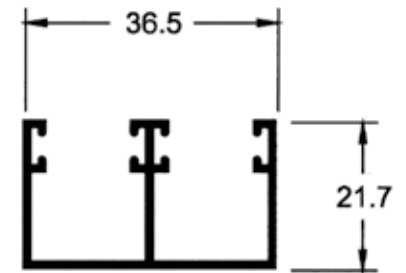
M - 6/B (8mm) 0,533 kg/m
